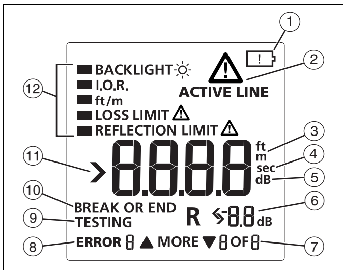
Figure 3. Display Features
